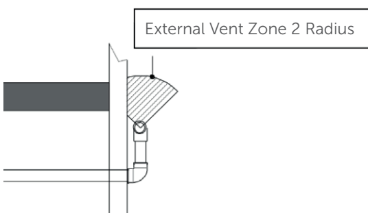
Hyprolyser 180-8500: Ventilation Zone 2 Radius
